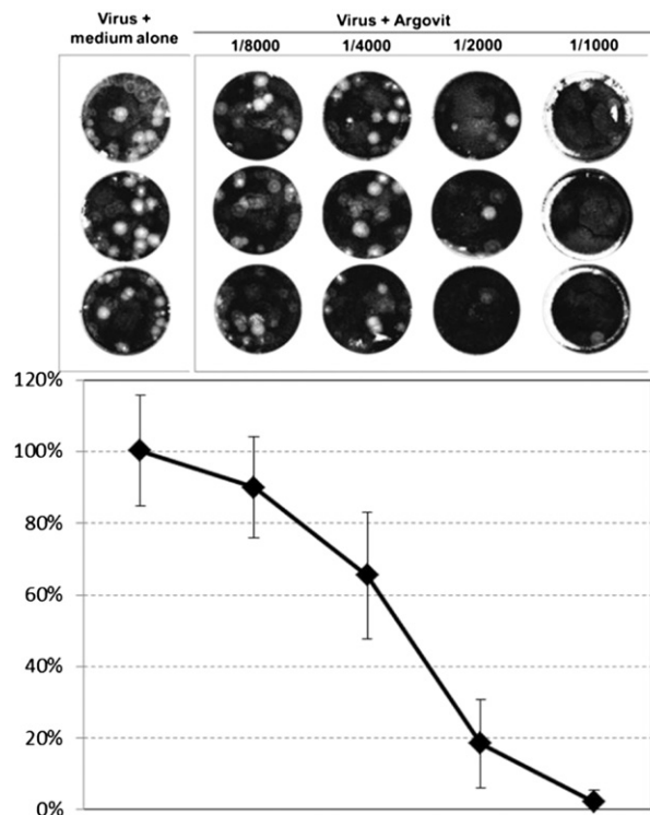
Figure 3. Reduction in the infectivity of RVFV MP12 by preincubation with Argovit. A fixed amount of virus was incubated with serial dilutions of Argovit or with medium alone, and then plaqued onto Vero cell monolayers. Cells were fixed and stained at 5 dpi and plaques counted to calculate the percentage of infectivity reduction reached at the different conditions assayed.
